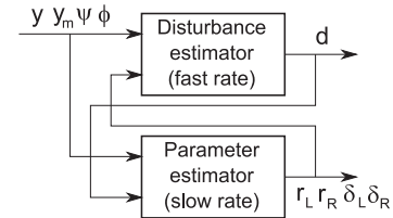
Fig. 8. Looped estimator
